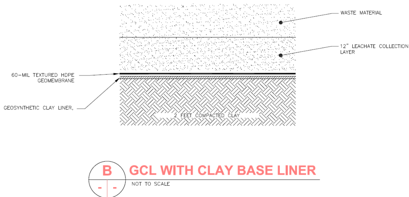
Figure 2: GCL with two feet of Clay Base Liner
