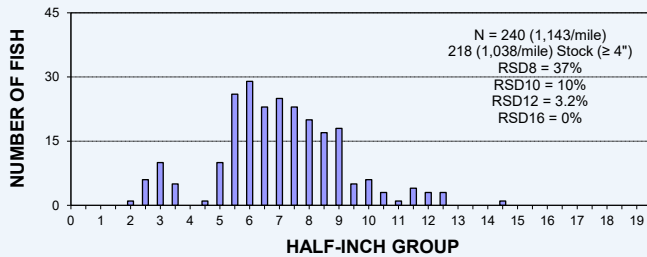
EAST BRANCH EAU CLAIRE RIVER HABITAT BELOW CTH C - 2024 BROOK TROUT LENGTH FREQUENCY
