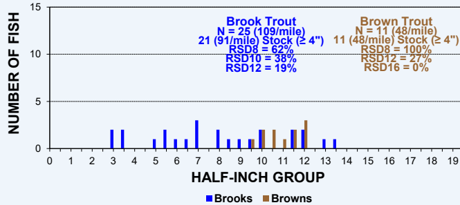
NINEMILE CREEK UPSTREAM FROM EAST HOLLISTER ROAD - 2024 BROOK & BROWN TROUT LENGTH FREQUENCIES
