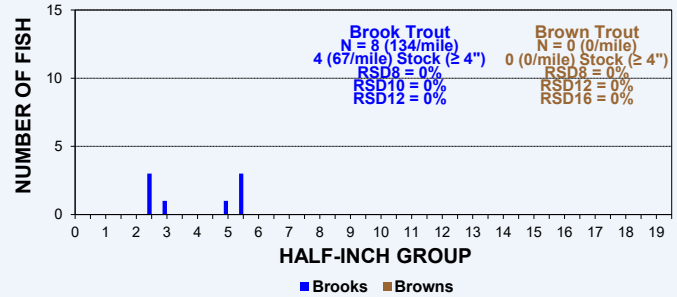
NINEMILE CREEK DOWNTOWN FROM STH 55 - 2024 BROOK & BROWN TROUT LENGTH FREQUENCIES
