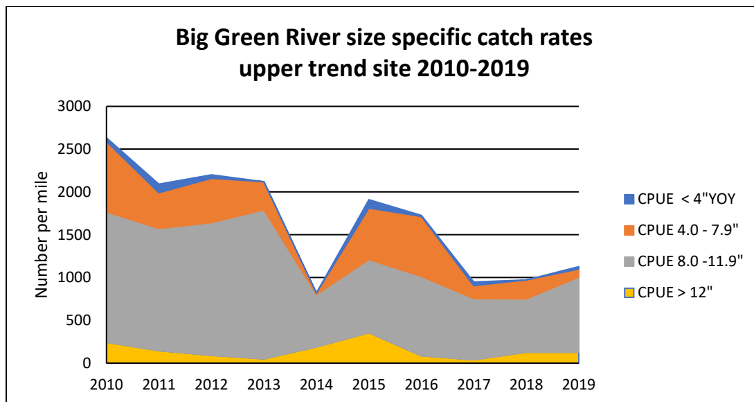
Figure 10. Big Green River upper trend station Brown Trout catch per unit effort 2010 – 2019.
