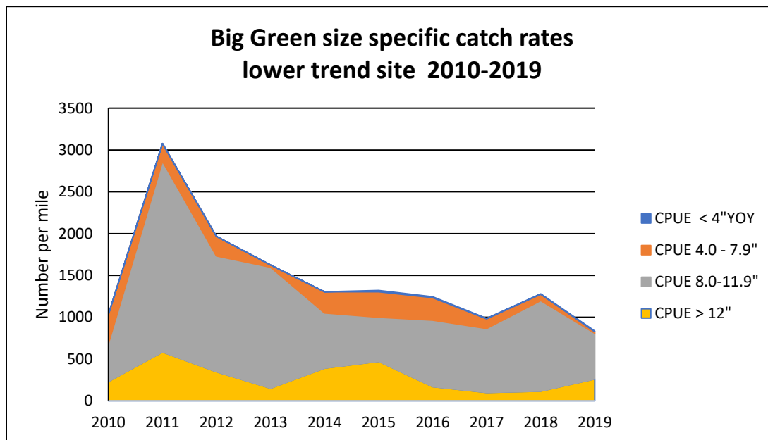
Figure 11. Big Green River lower trend station Brown Trout catch per unit effort 2010 – 2019
