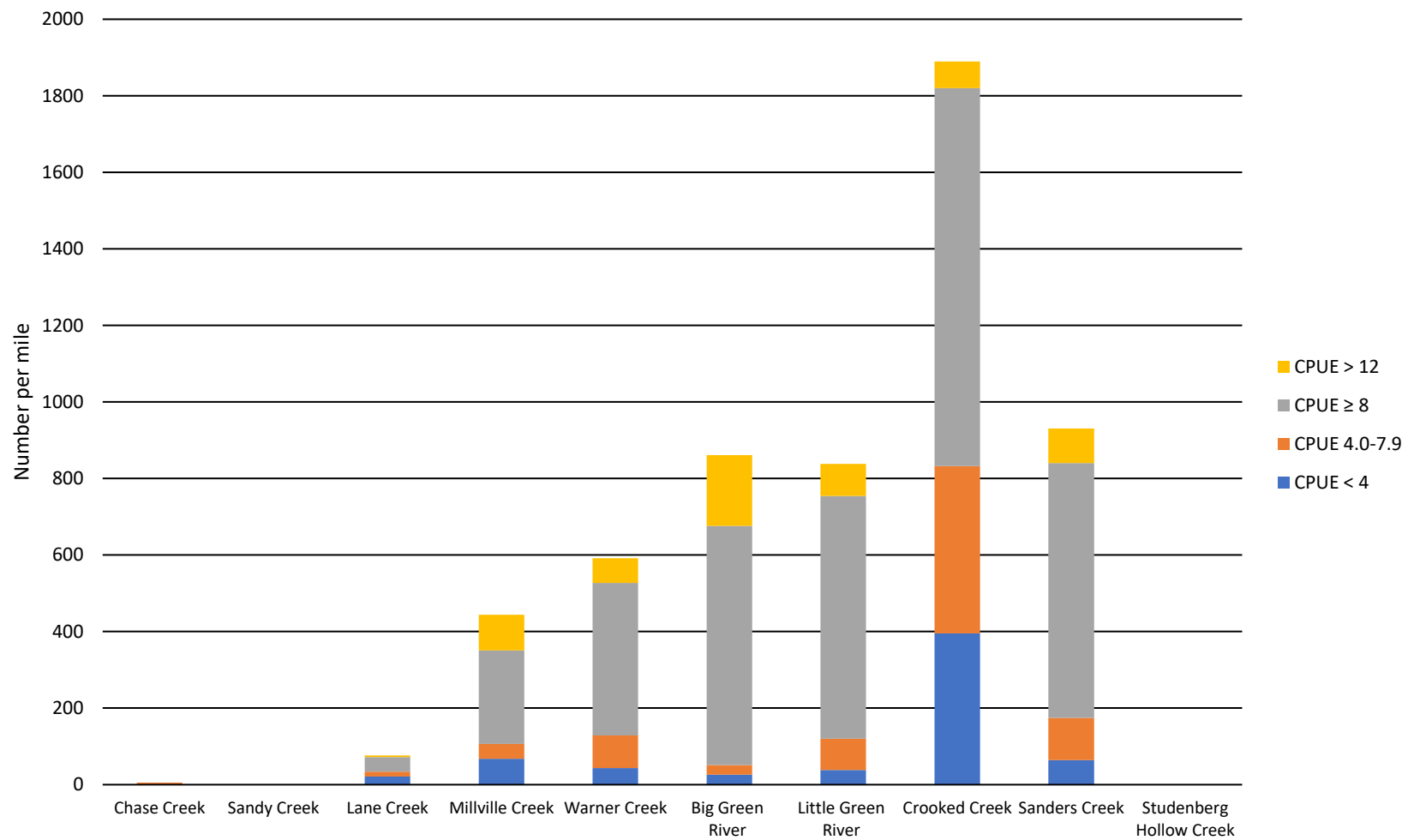
Figure 4. Brown Trout catch per unit effort by stream.
