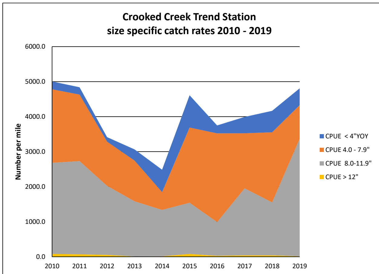
Figure 9. Crooked Creek trend station Brown Trout catch per unit effort 2010 – 2019.
