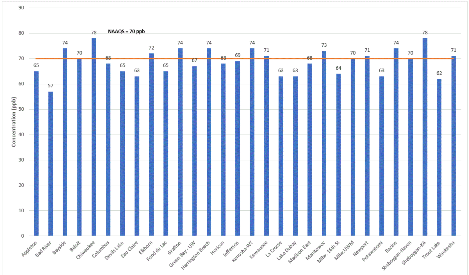
Figure 7: 8-hour Ozone 2022 – 2024 Design Values Compared to the NAAQS
